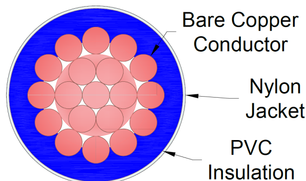
Drawing of 1/0AWG THHN/THWN-2
